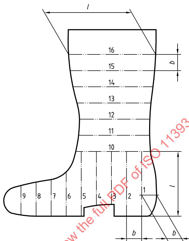
Figure 2 — Cross-sections of an artificial boot (in the central plane)
