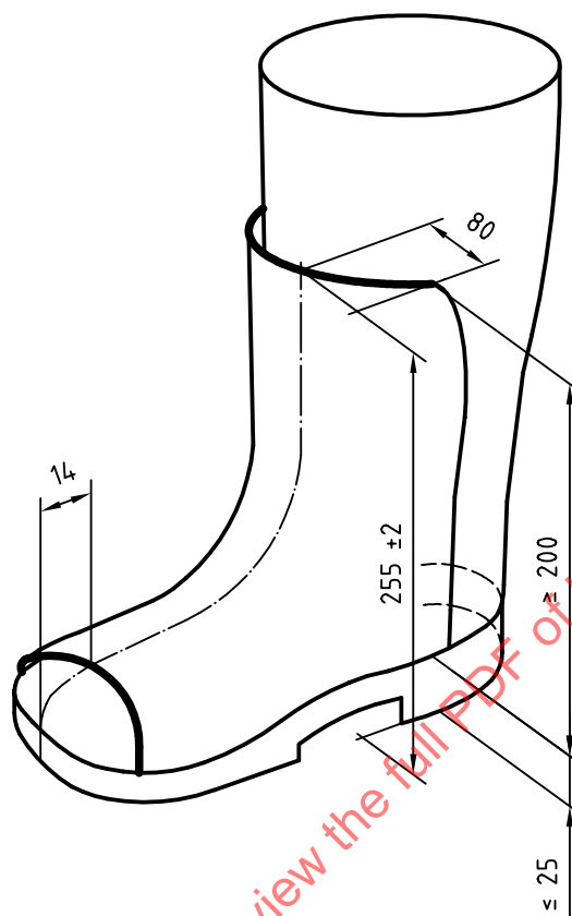
Figure 1 — Specified protective area (as marked on the artificial boot)
