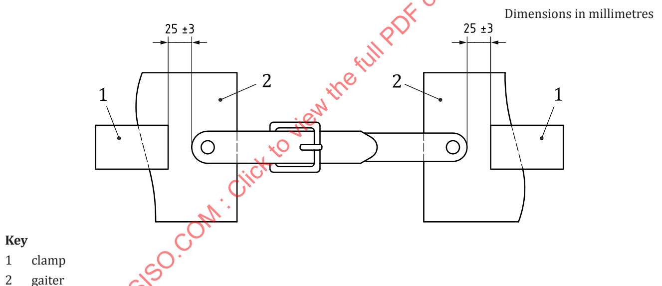
Figure 2 — An example for testing the strength of fastening systems
