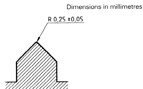
Figure 3 — Prism used in the test device for measuring balance point
