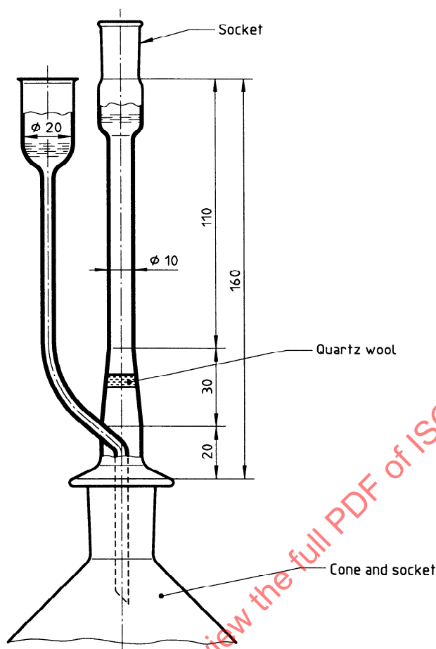
Figure 1 — Microseparator
