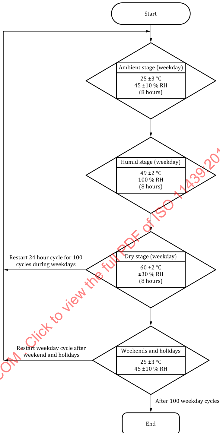
Figure H.1 — Accelerated cyclic corrosion flow diagram
