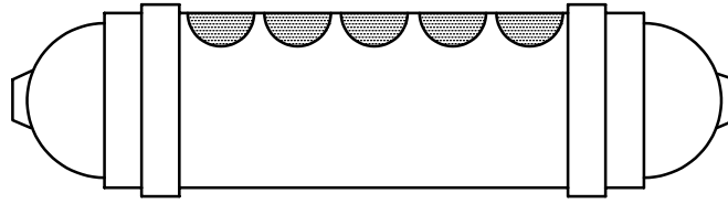
Figure A.1 — Cylinder orientation and layout of exposure areas
