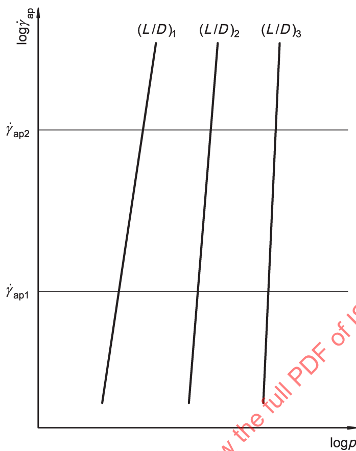
Figure 3 — Application of the Bagley correction method [3] — Plot of the apparent shear rate \dot{\gamma}_{ap} versus the test pressure p for different values of L/D
