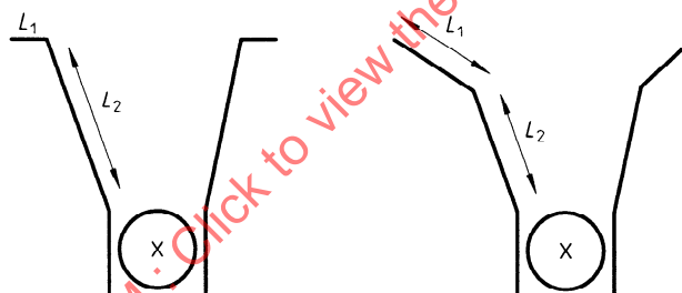
Figure 3 — Chain measurement
