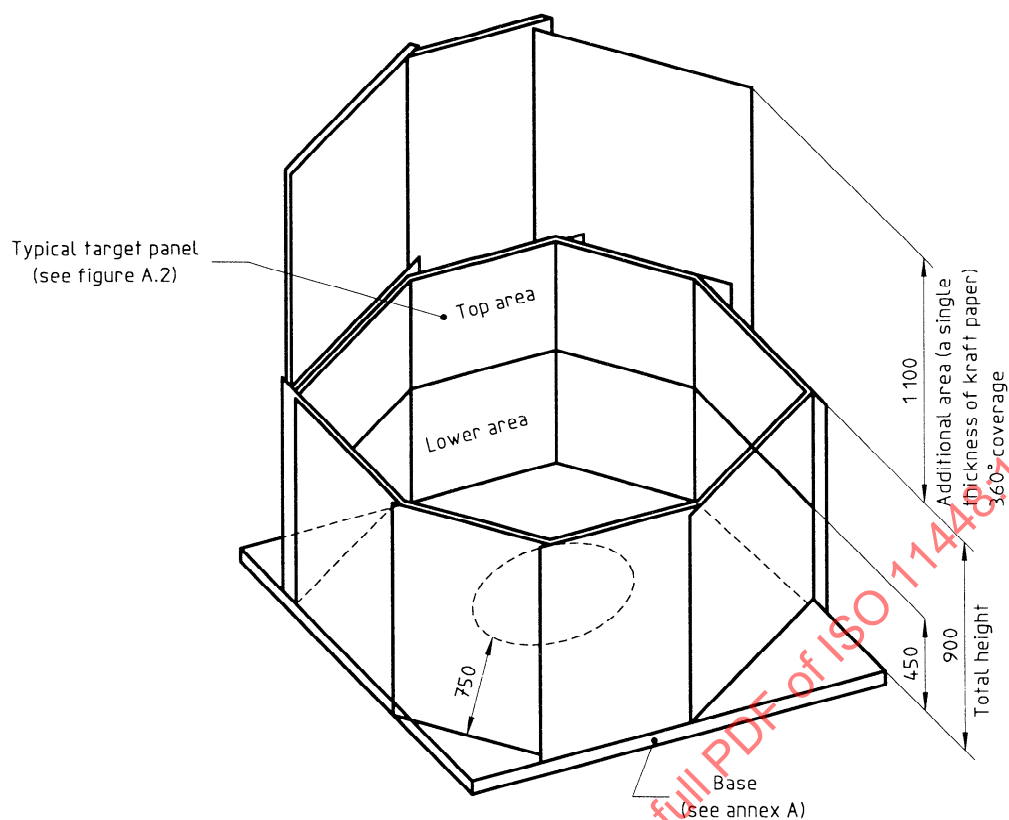
Figure 7 — Thrown object test figure — General layout
