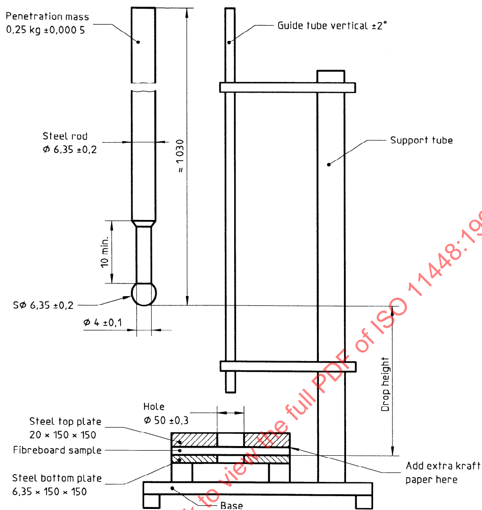
Figure B.1 — Test fixture for corrugated fibreboard penetration test
