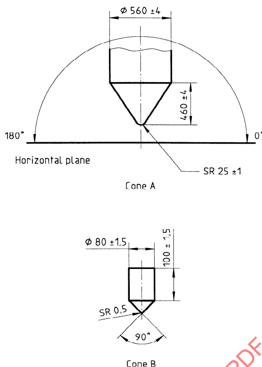
Figure 6 — Test cones
