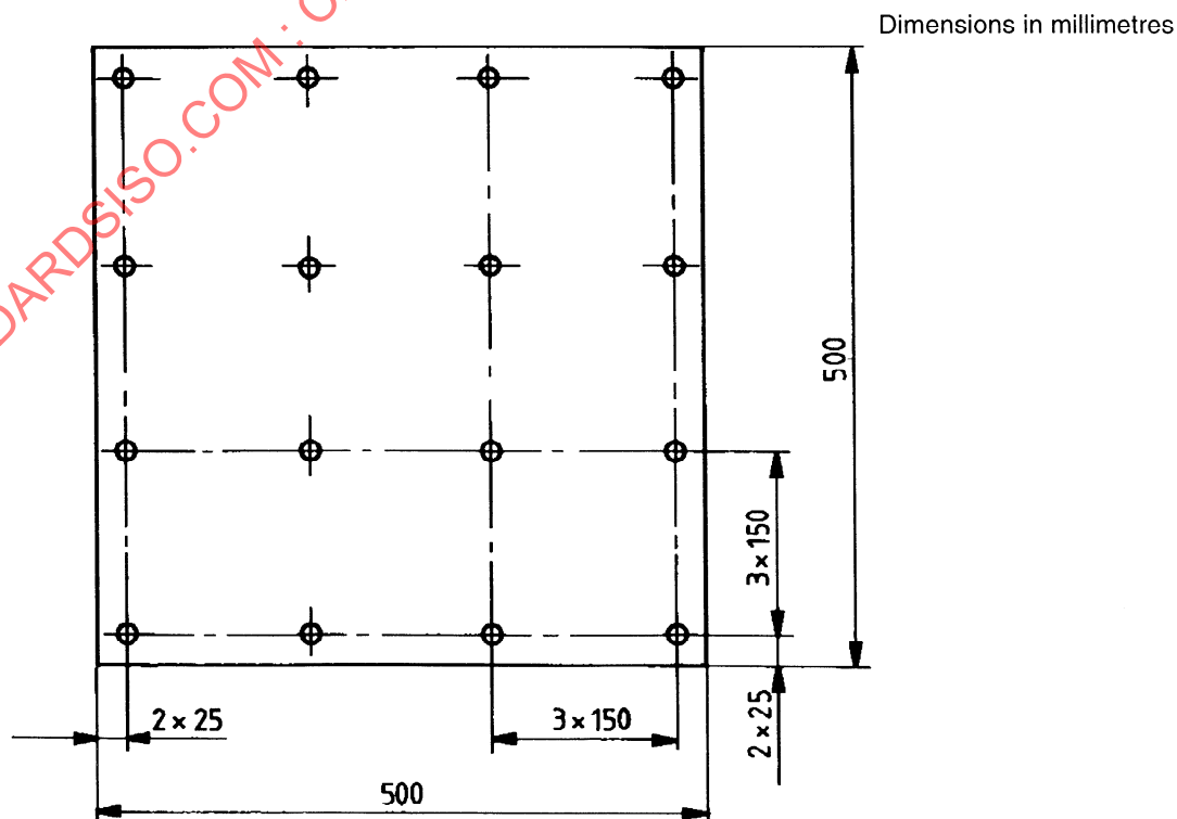
Figure A.1 — Nail plan of test fixture base
