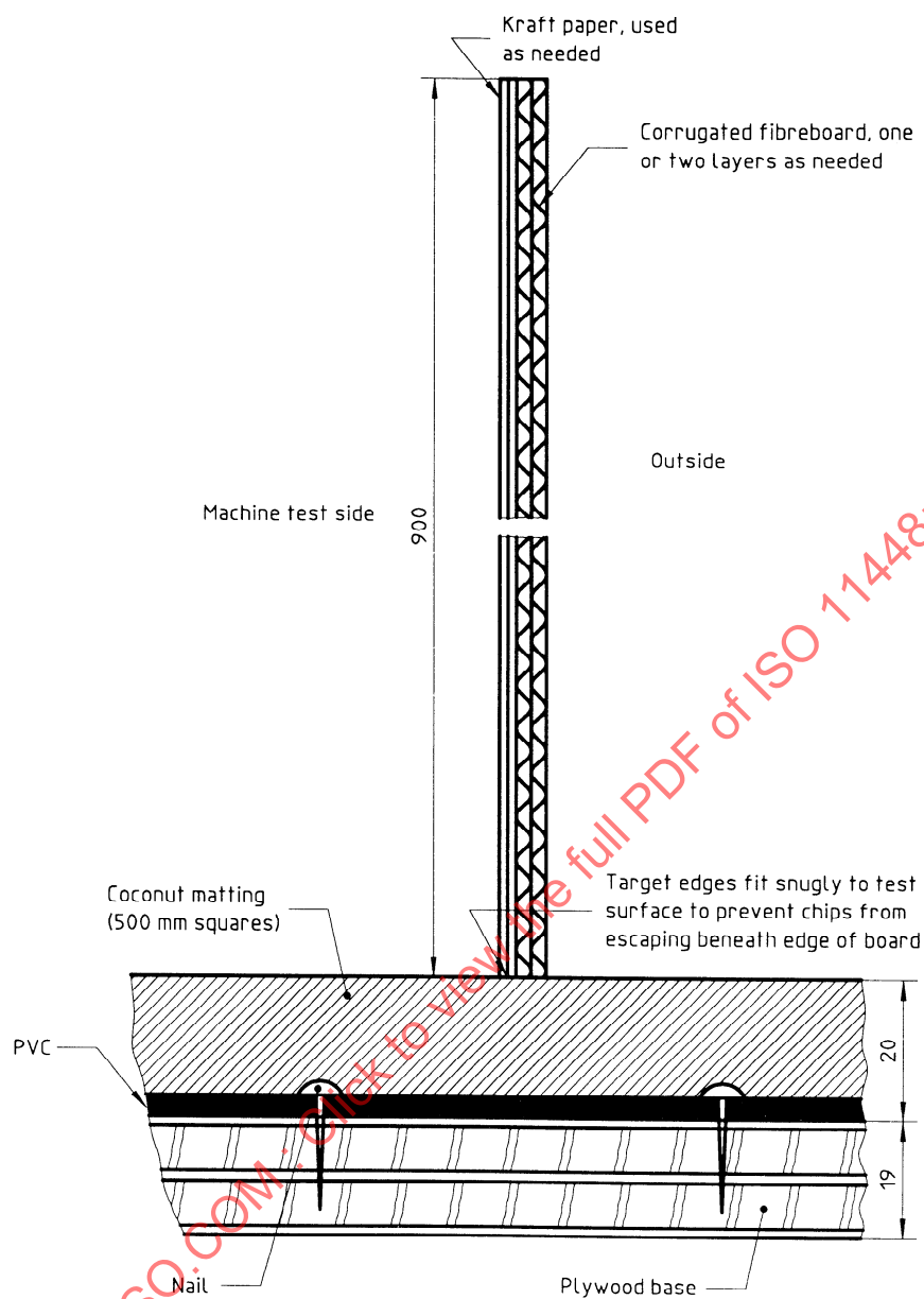
Figure A.2 — Test enclosure walls and base
