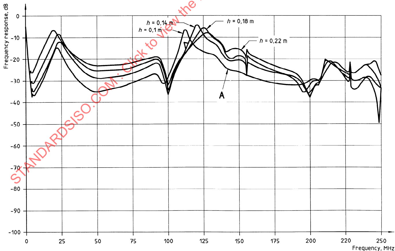
Figure B.5 — Line coupling of a stripline inside a TEM cell for different heights, h
