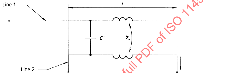
Figure B.1 — Coupling between transmission lines
