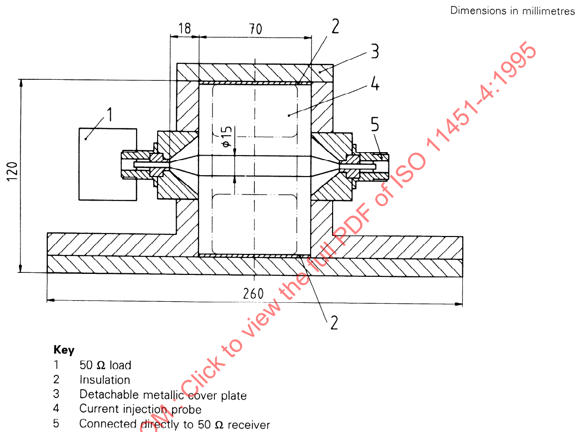
Figure A.2 — Current injection probe calibration fixture
