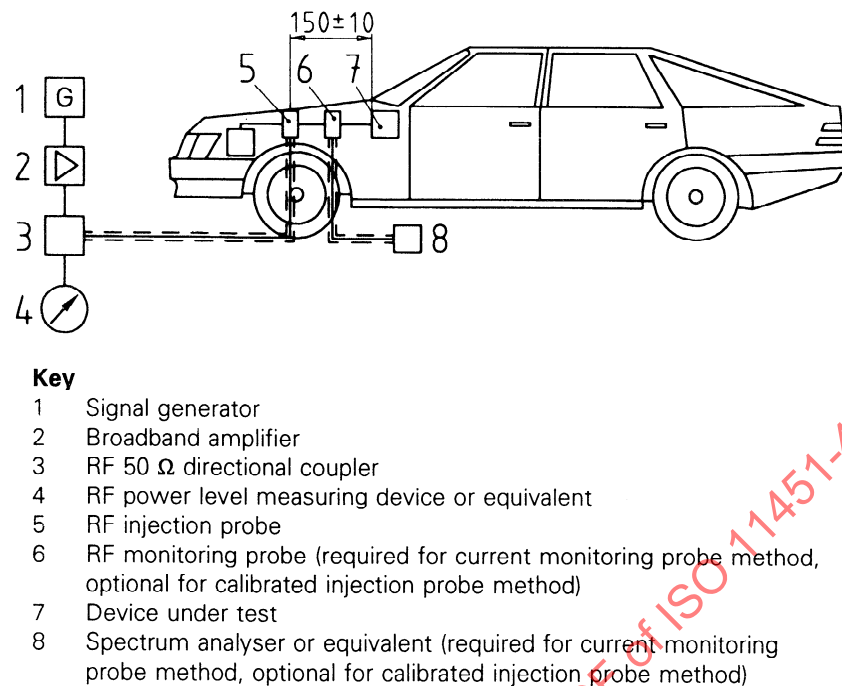
Figure 1 — Example of BCI test configuration
