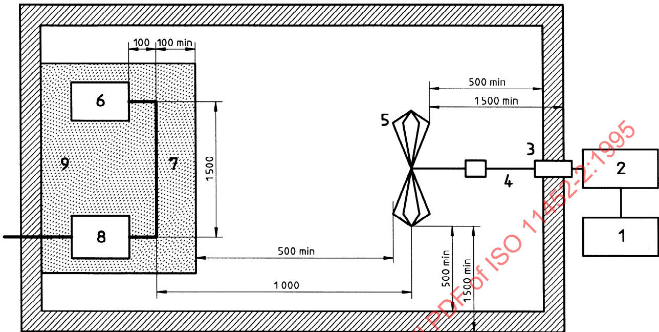
a) Top view (horizontal polarization)
