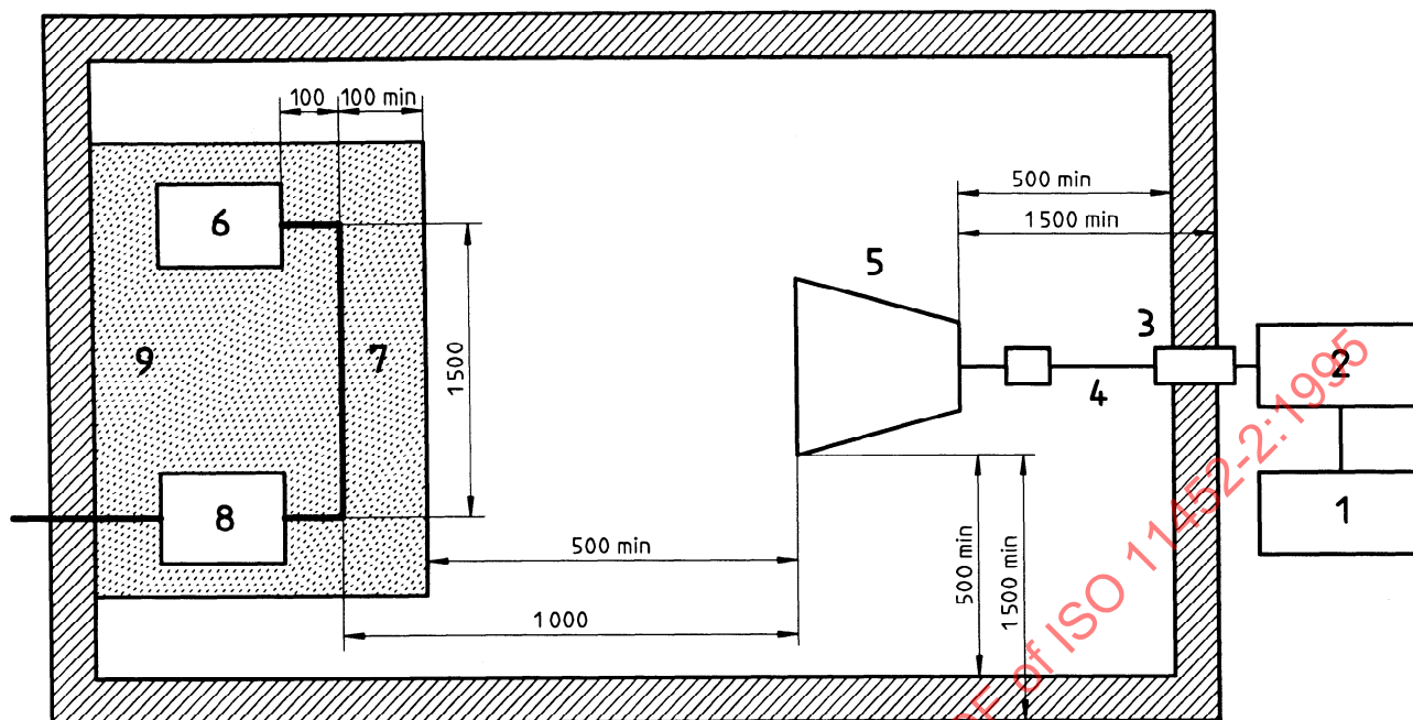
a) Top view (horizontal polarization)
