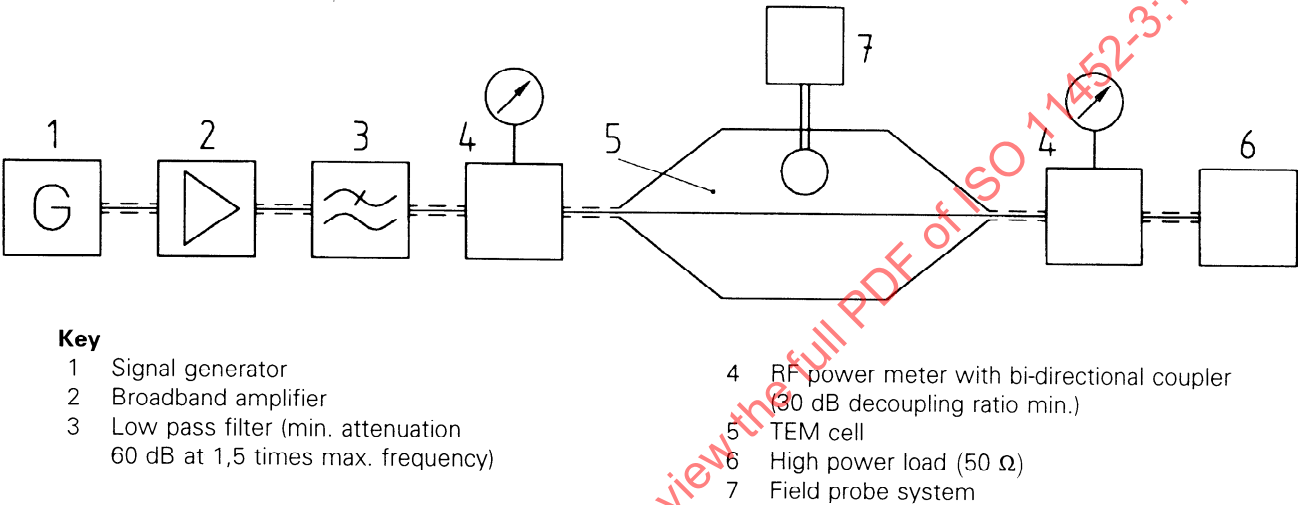
Figure A.1 — Block diagram of field probe system calibration
