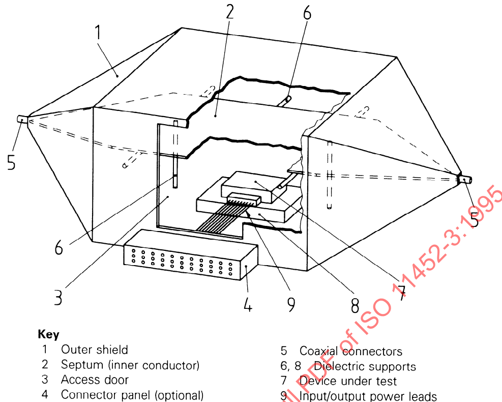
Figure 1 — TEM cell
