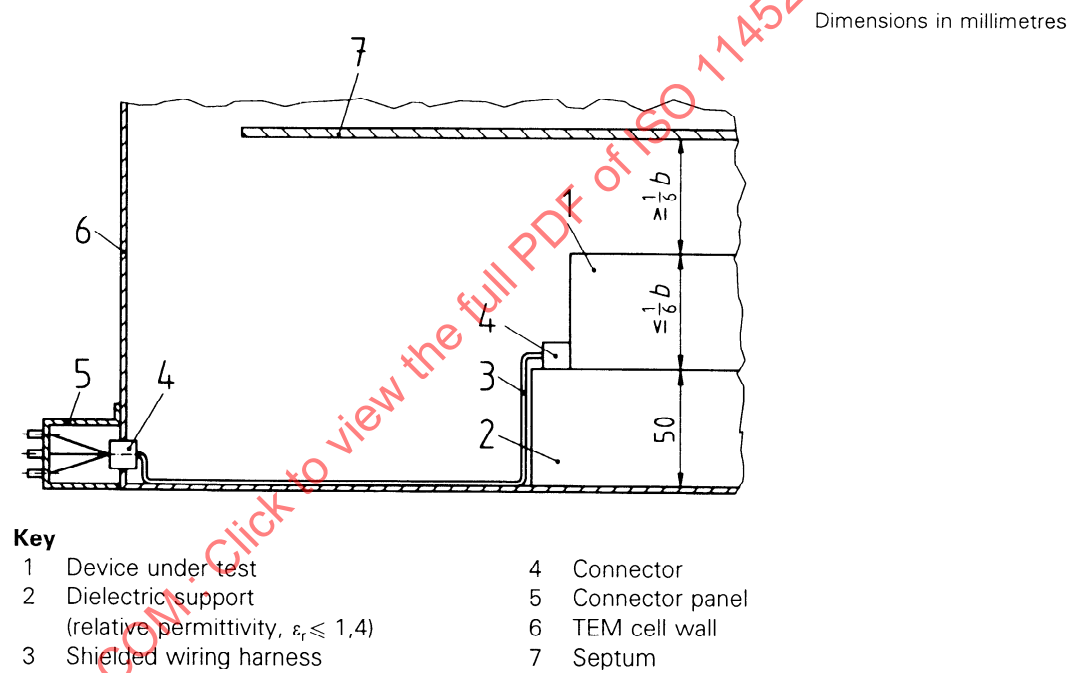
Figure 5 — Example of test set-up
