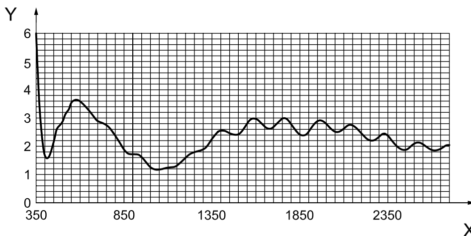
Figure B.1 — Typical VSWR characteristics
