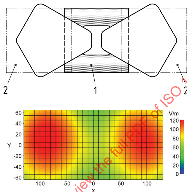
400 MHz; 1 W net; average field strength: 100 V/m
