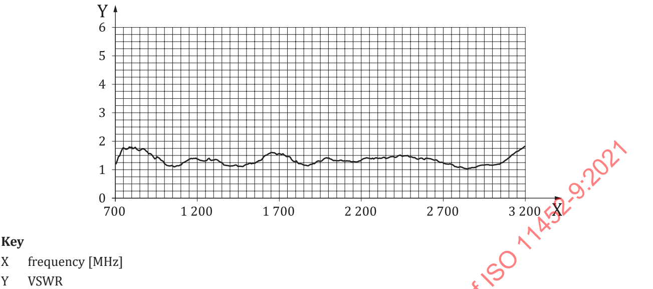
Figure C.4 — Typical VSWR characteristics of broadband sleeve antenna
