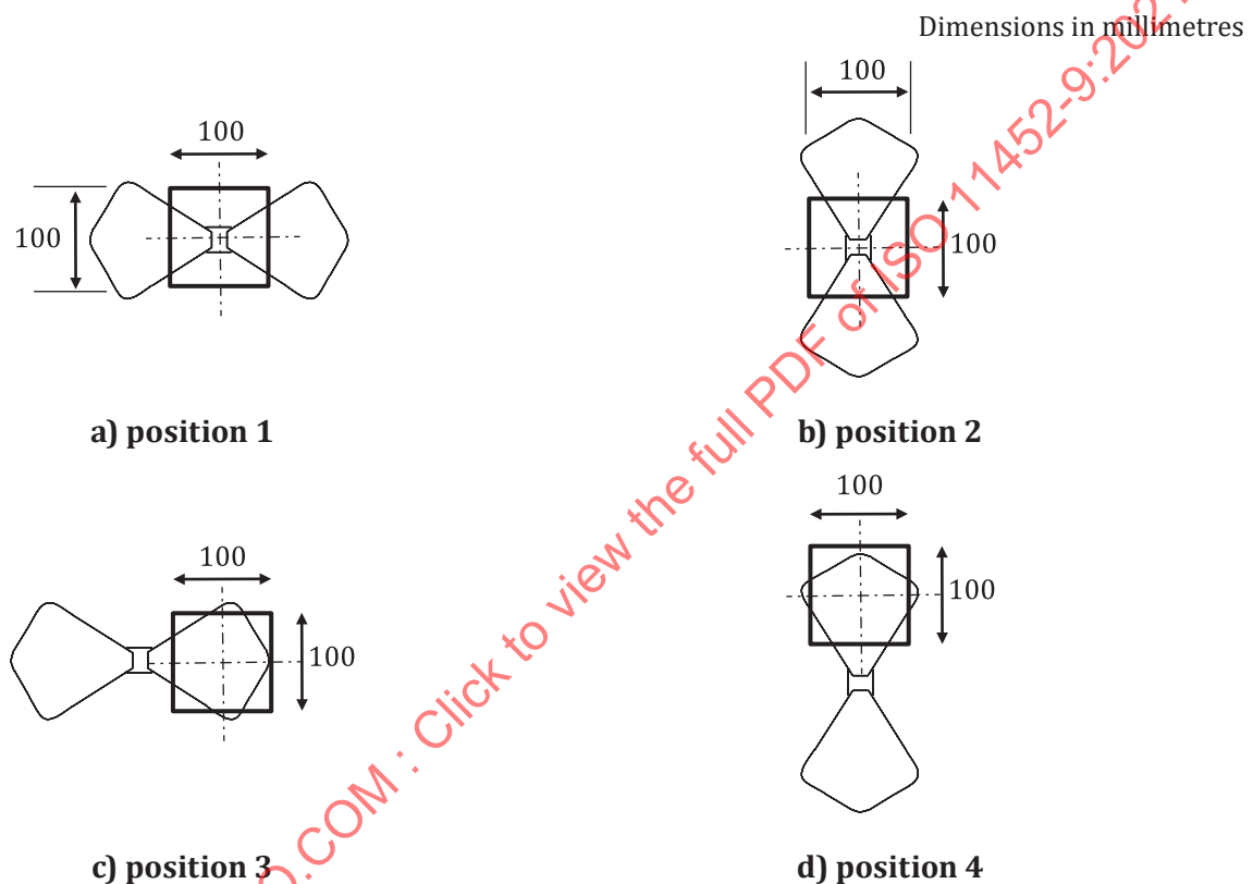
Figure 11 — Method 1 testing with broadband dipole antenna
