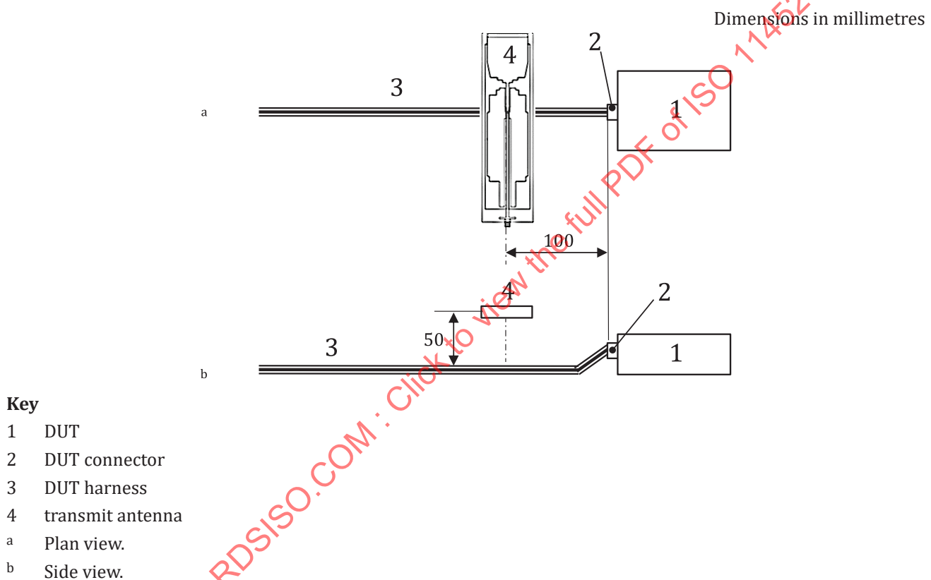
Figure 19 — Initial location broadband sleeve antenna for harness coupling
