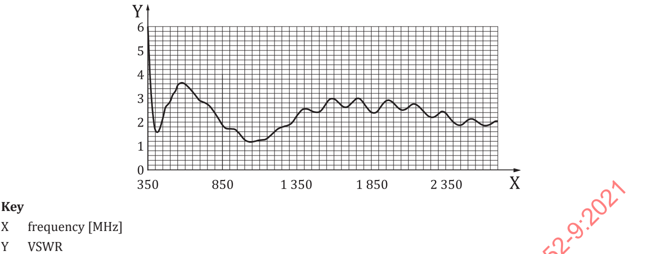
Figure C.1 — Typical VSWR characteristics of broadband dipole antenna
