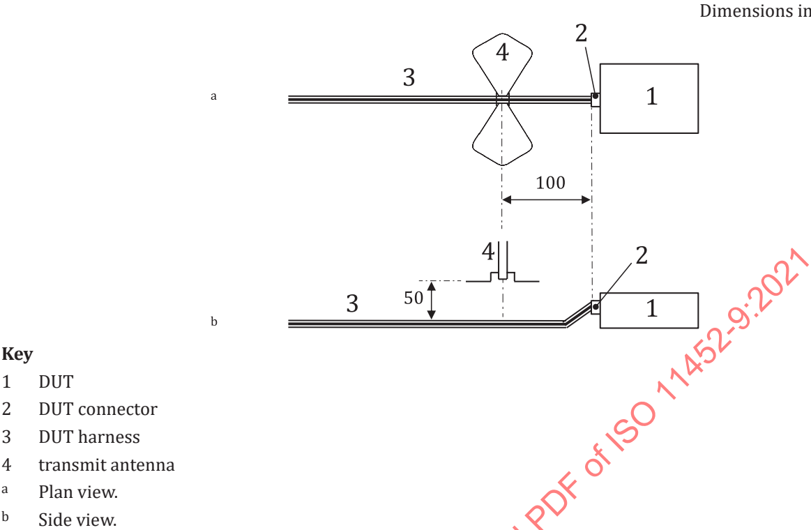
Figure 17 — Initial location of broadband dipole antenna for harness coupling
