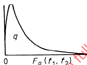
Figure 1 — Quantiles of the F -distribution
