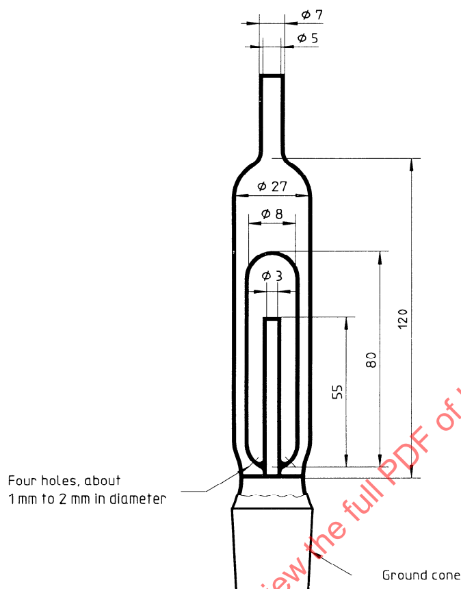
Figure 2 — Example of an absorption vessel
