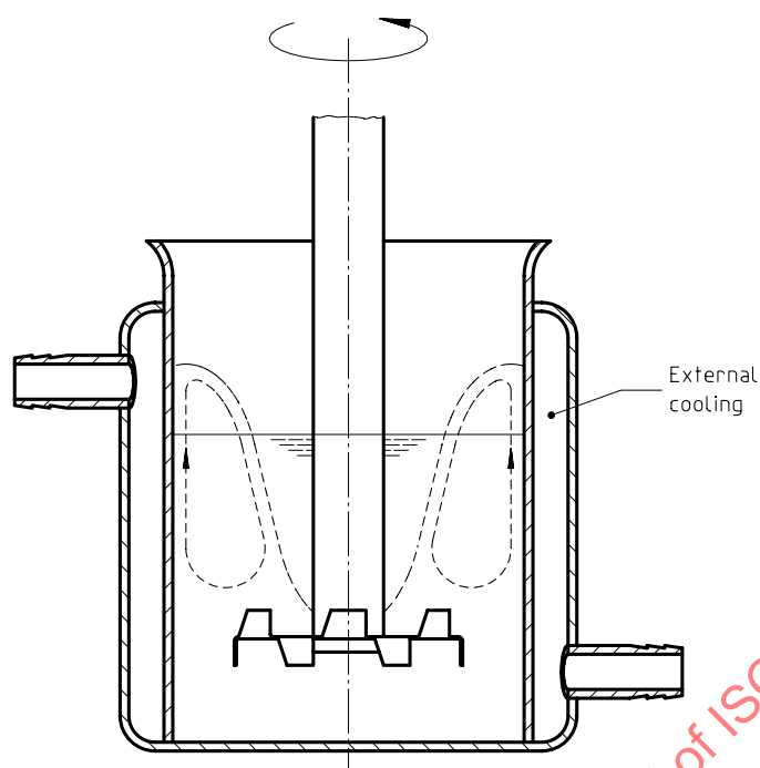
Figure 1 — Dissolver (double-walled)
