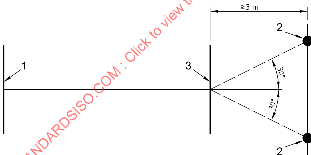
Figure 1 — Schematic for reflected light observation of coated glass
