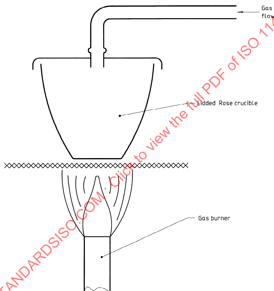
Figure A.1 — Reduction apparatus
