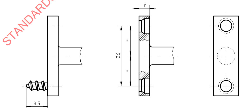
Figure 5 — Attachment element
