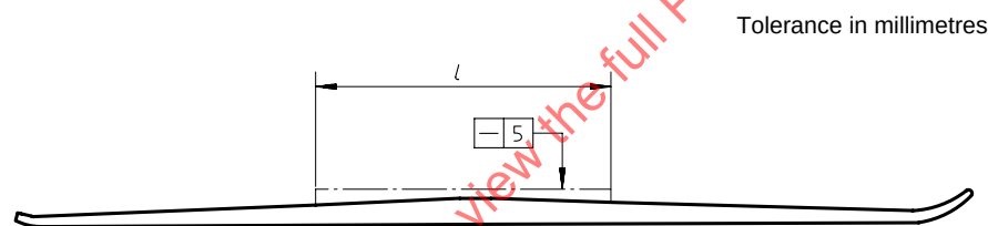
Figure 2 — Longitudinal profile of the surface
