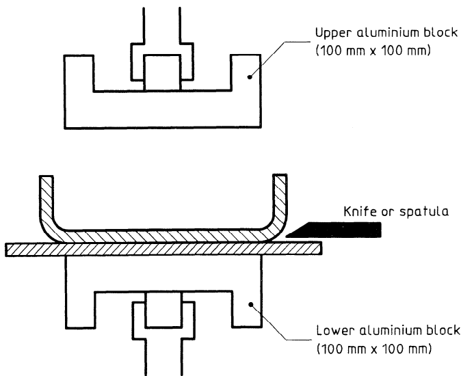
Figure 4 — Fixing blocked specimens to aluminium blocks in quantitative method (method B)
