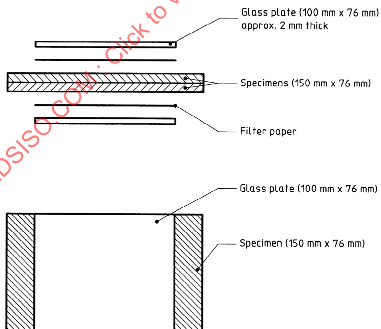
Figure 3 — Assembly of specimens for quantitative method (method B)
