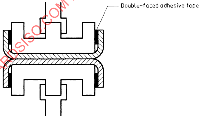
Figure 5 — Specimen in test position in quantitative method (method B)
