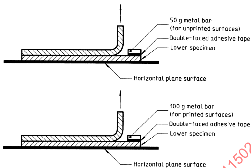
Figure 2 — Separation of specimens in qualitative method (method A)
