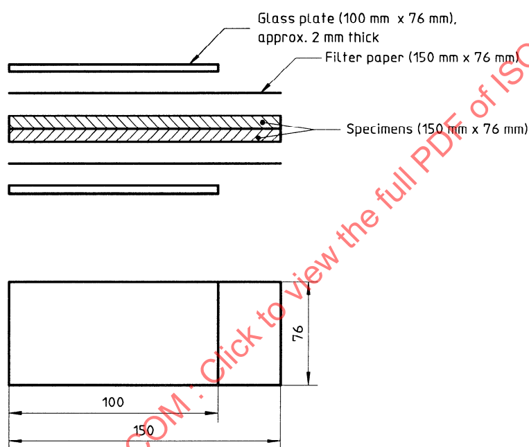
Figure 1 — Assembly of specimens for qualitative method (method A)
