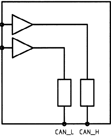
Figure 18 — Termination network
