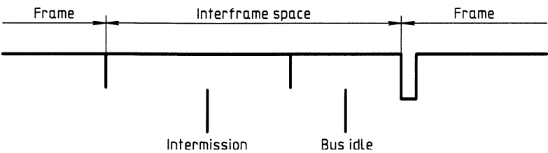
Figure 9 — Interframe space for nodes which are not “error passive” or have been a receiver of the previous frame
