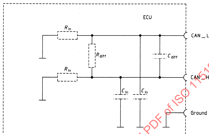
Figure 1 — Definitions of internal capacitances and internal resistances of an ECU
