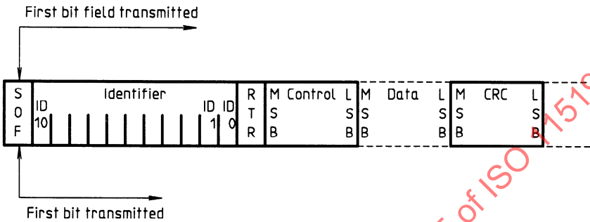
Figure 12 — Order of bit transmission
