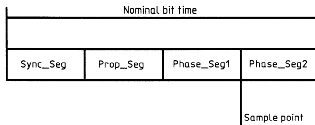
Figure 14 — Partition of the bit time
