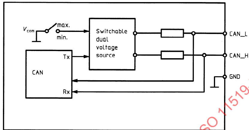
Figure 24 — Structure of the test transmitter
