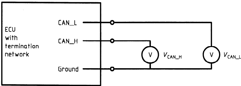
Figure 19 — Measurements of V_{CAN\_L} and V_{CAN\_H} during the bus idle state
