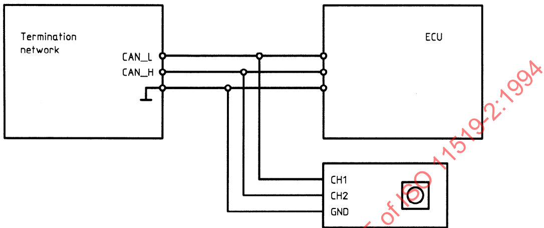
Figure 22 — Measurements of V_{CAN\_L} and V_{CAN\_H} while the ECU is sending a dominant bit
