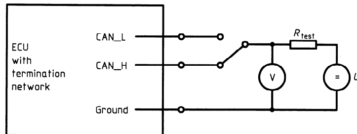
Figure 20 — Measurement of R_{in} of ECU with termination network
