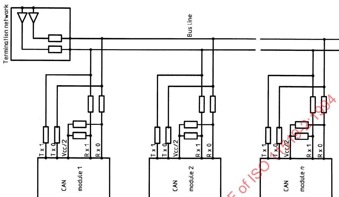
Figure 15 — Suggested electrical interconnection
