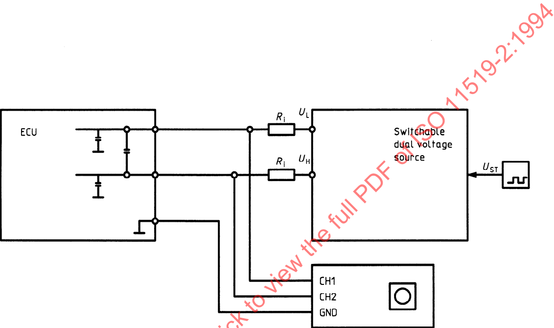
Figure 25 — Measurement of the input capacitance C_{busin} during the recessive state
