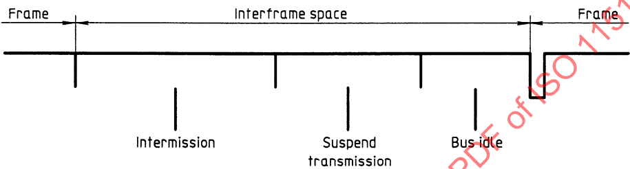
Figure 10 — Interframe space for “error-passive” nodes which have been a transmitter of the previous frame
