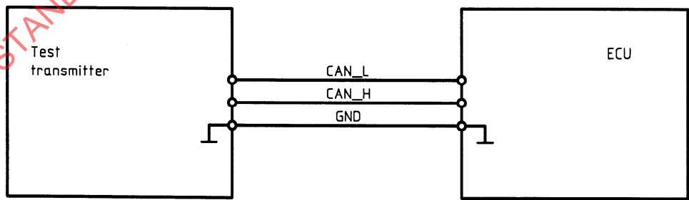
Figure 23 — Testing of the input threshold during transmission
