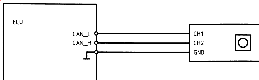
Figure 21 — Measurements of V_{CAN\_L} and V_{CAN\_H} while the ECU is sending a dominant bit
