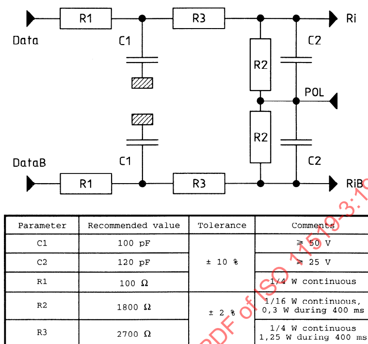
Figure 53 — 250 kTS/s filter
