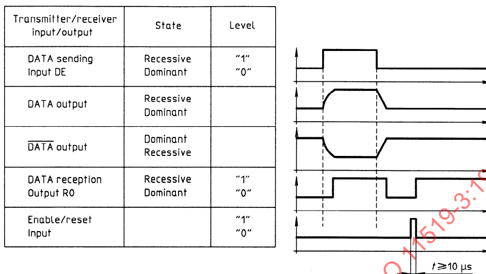
Figure 51 — Timing diagram
