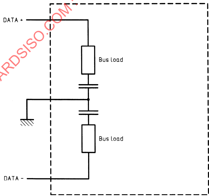
Figure 50 — Option: Analog filter
