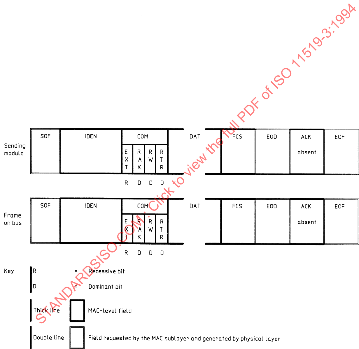
Figure 13 — Structure of data frames without request for acknowledgement — Enhanced Manchester
