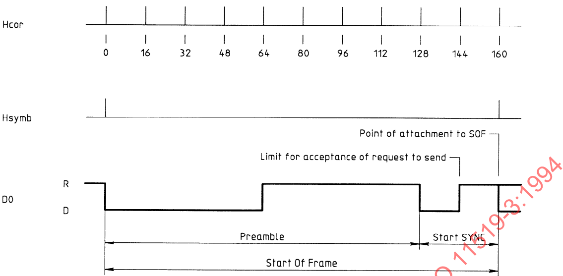
Figure 36 — Description of Start Of Frame (SOF) delimiter — Manchester-L and Enhanced Manchester
