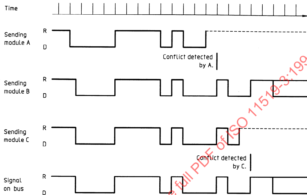
Figure 26 — Mechanism of bitwise arbitration on bus in Enhanced Manchester
