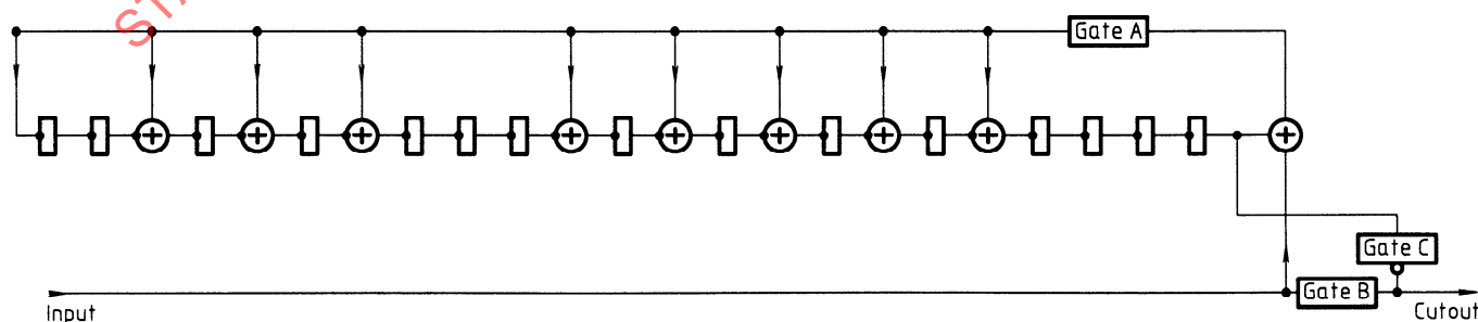
Figure 11 — Block diagram of Frame Check Sequence (FCS) encoder
