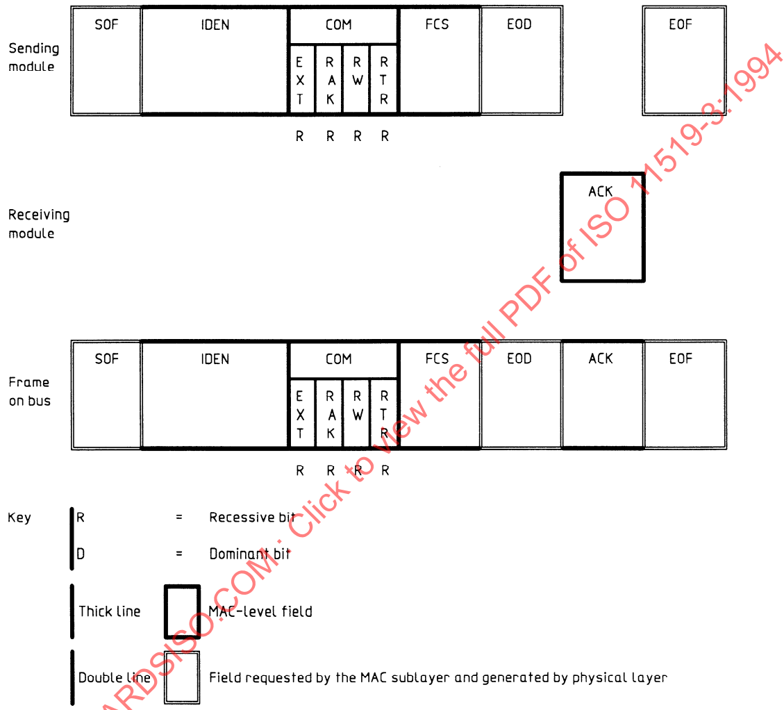
Figure 19 — Structure of remote transmission request and without in-frame response with acknowledgement — Enhanced Manchester
