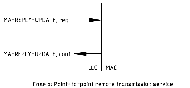
Figure 7 — Exchange of response preparation service primitives
