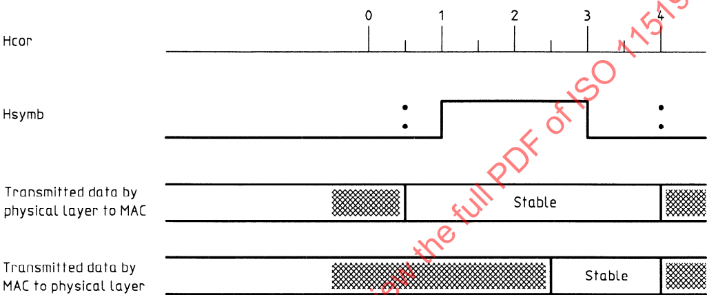
Figure 40 — Information exchange rule between MAC sublayer and physical layer
