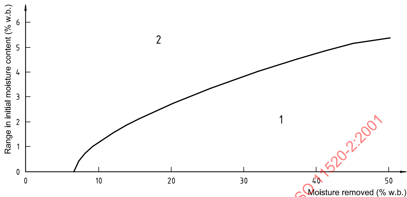
Figure A.3 — Relationship between moisture removed and range in variation in grain moisture content for a confidence level on evaporation rate of \pm 5\% or better at the 95 % level of probability
