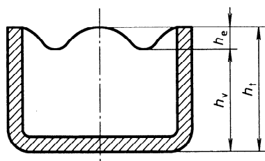
Figure 1 — Schematic section of cup
