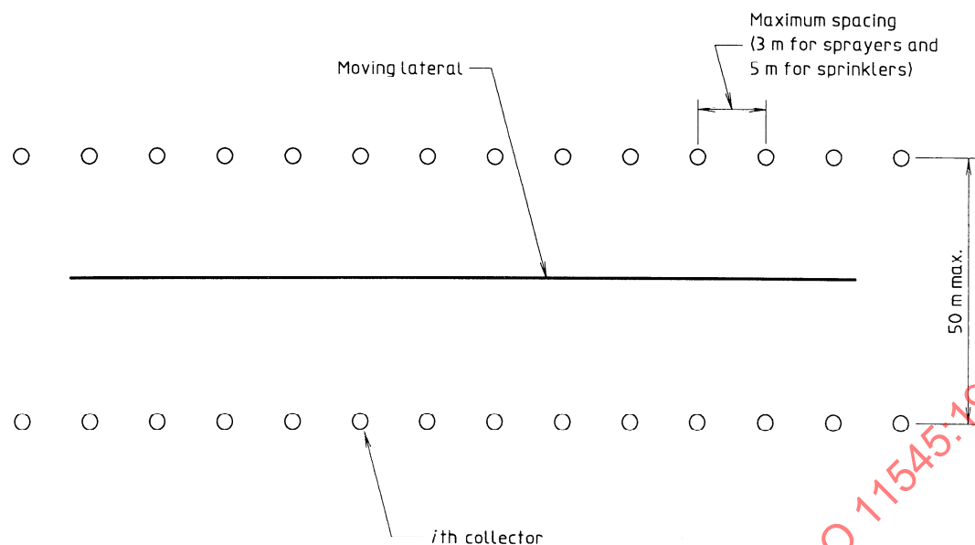
Figure 2 — Collector layout for determining water distribution of moving lateral irrigation machines
