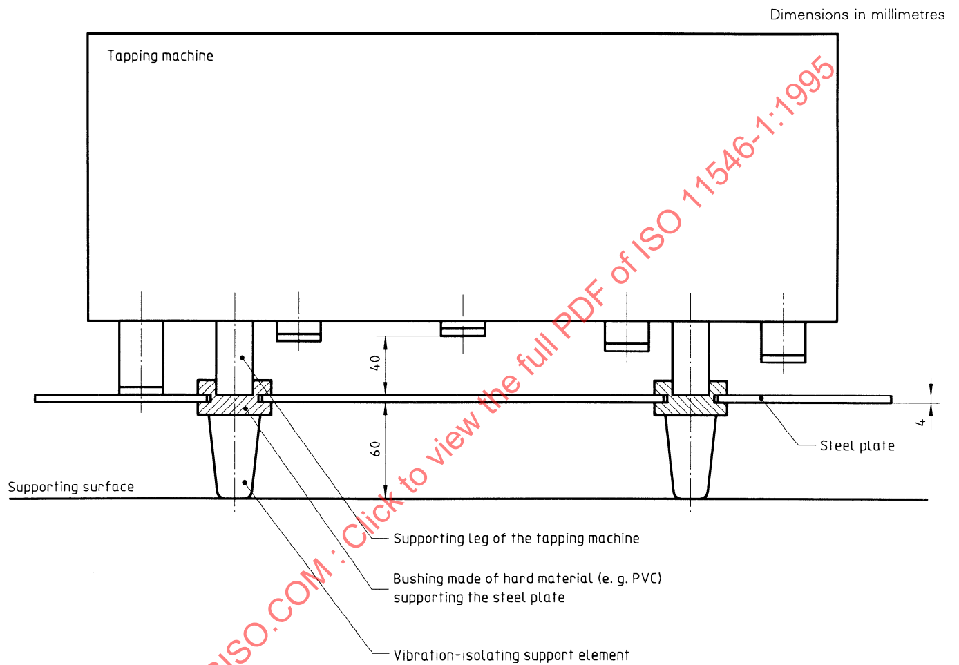
Figure A.1 — Artificial sound source (schematic)
