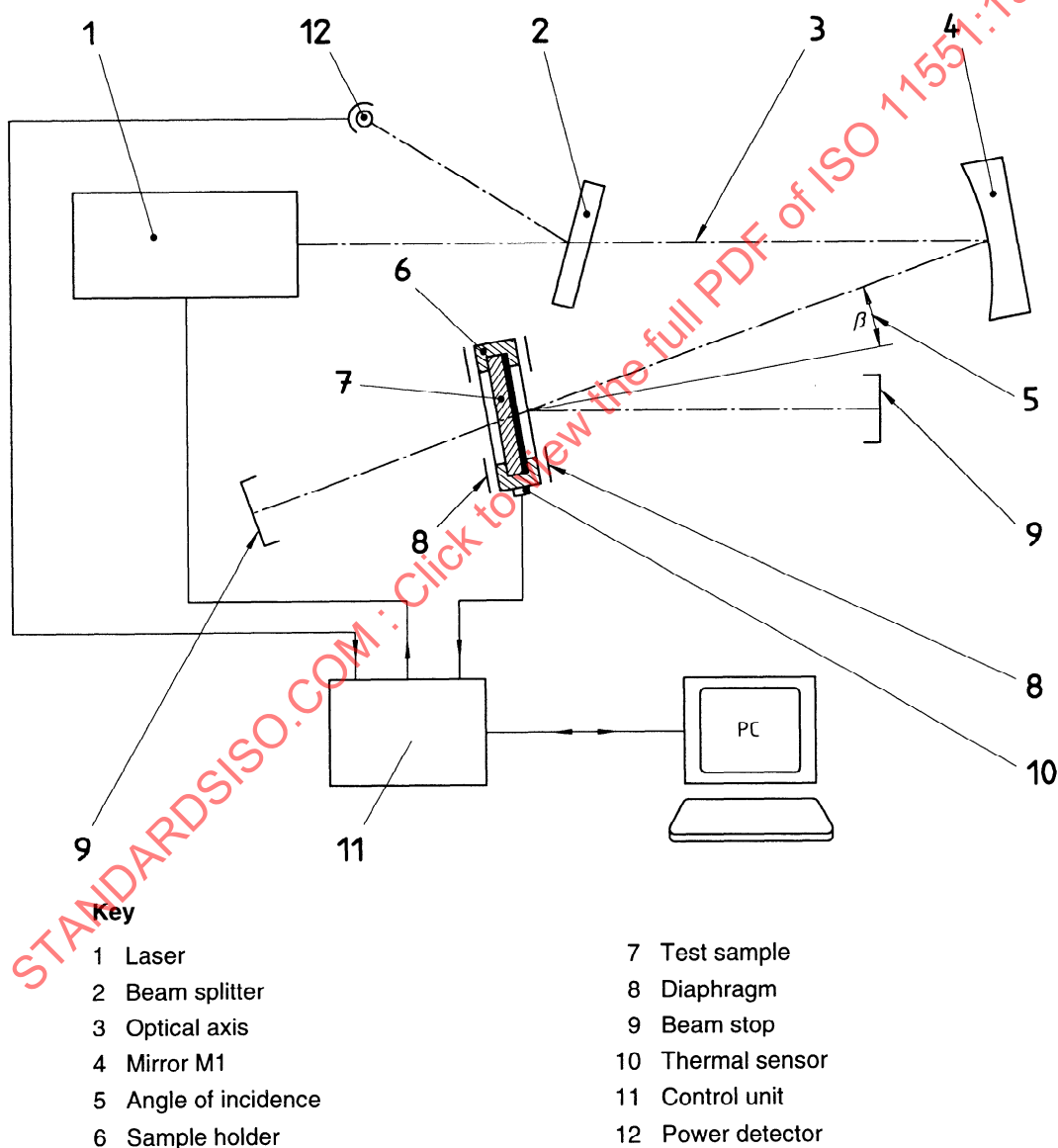
Figure 1 — Arrangement for measurement of the absorbance
