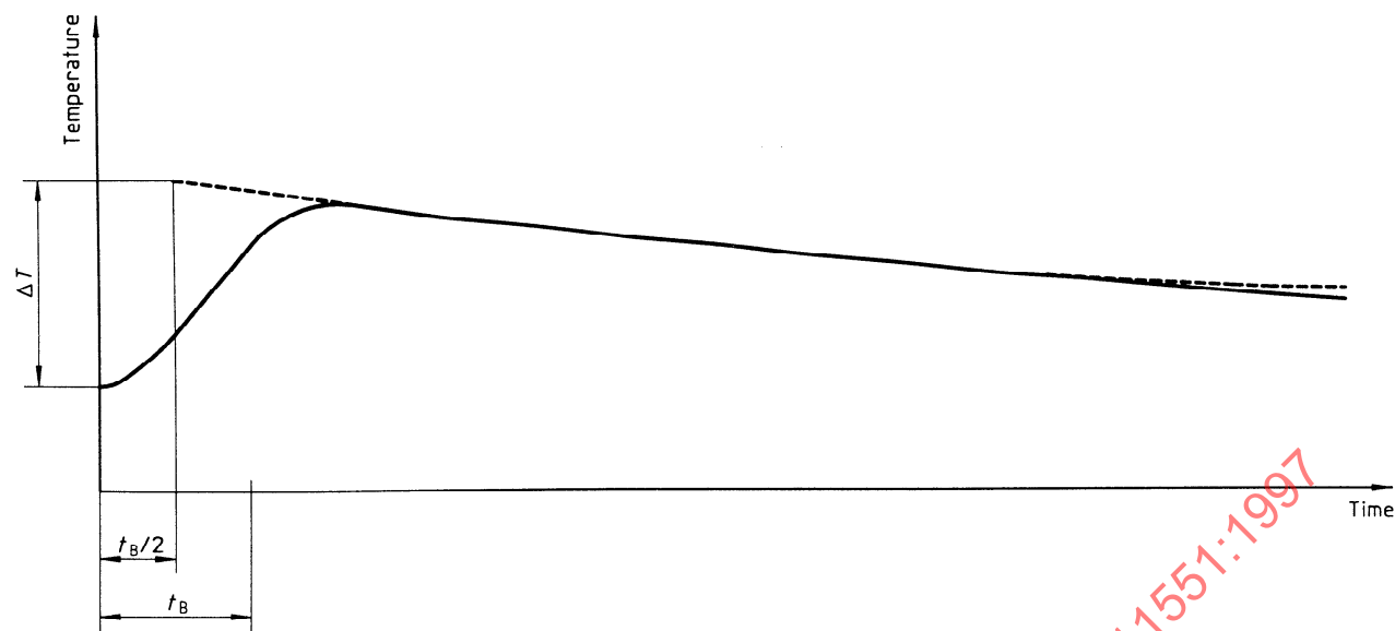
Figure 2 — Determination of absorbance, pulse method
