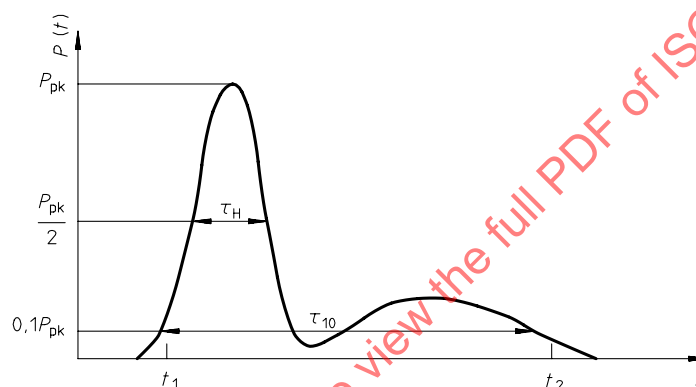
Figure 2 — Example of the variation of radiation power of the pulse of a TEA-laser with time
