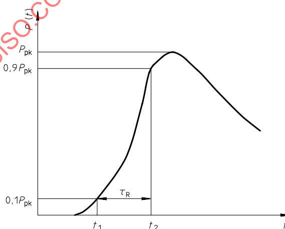
Figure 3 — Example of rise time measurement
