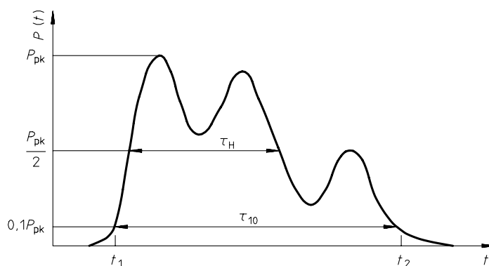
Figure 1 — Example of the variation of radiation power of a laser pulse with time
