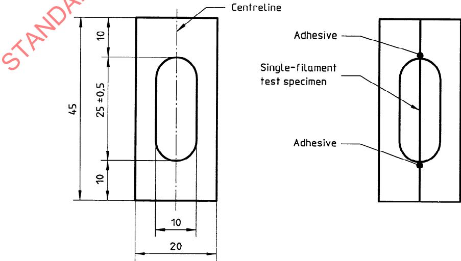
Figure 1 — Specimen mount and test specimen mounted on the mount
