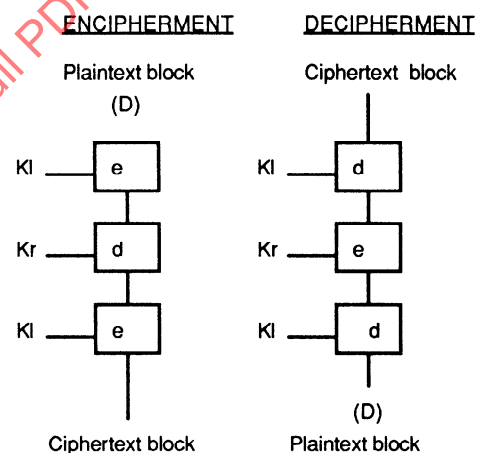
Figure 1 — Use of double length keys
