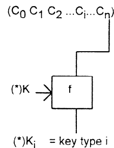
Figure 2 — Variant key calculation
