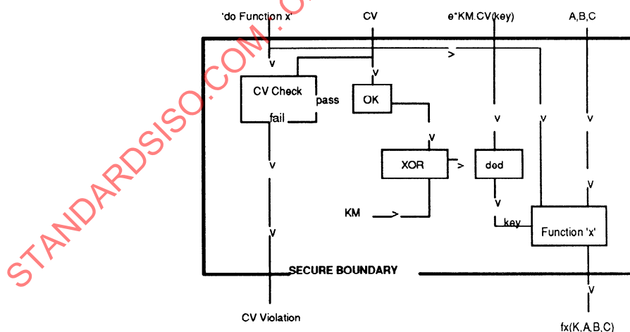
Figure E.1 — Example of Control Vectors for 'function x'
