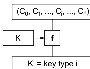
Figure 2 — Variant key calculation
