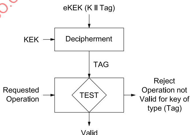
Figure 7 — Tagged key use
