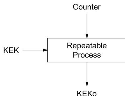
Figure 5 — Calculation of a KEK offset (KEKo)
