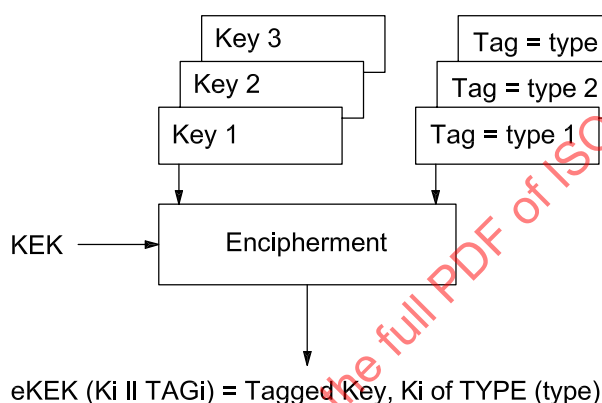
Figure 6 — Tagged key generation
