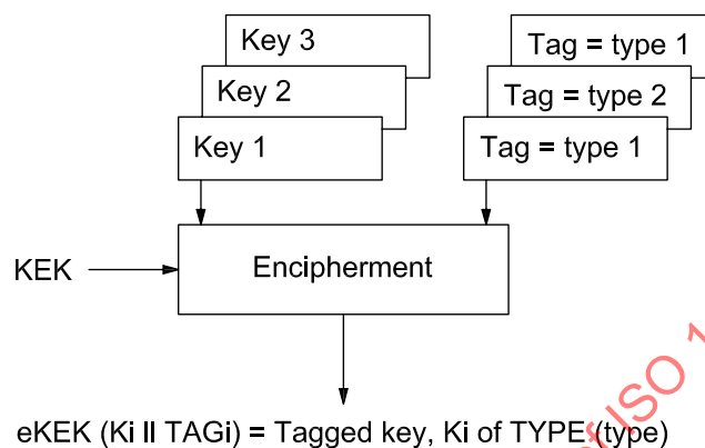
Figure 6 — Tagged key generation
