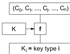
Figure 2 — Variant key calculation
