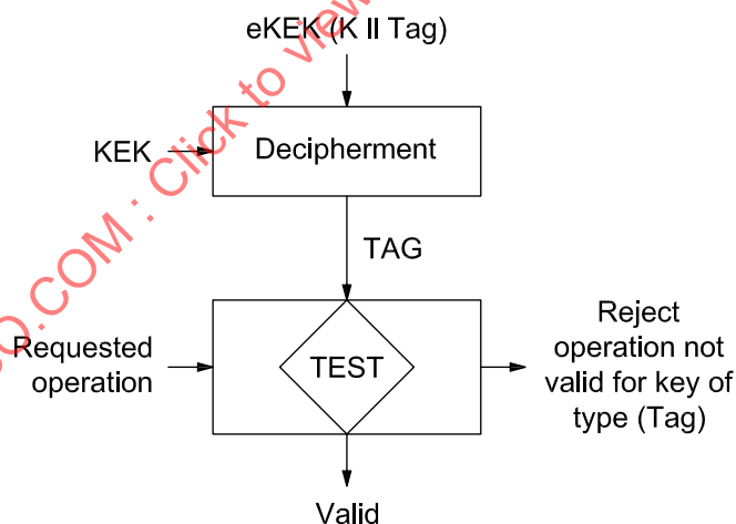
Figure 7 — Tagged key use
