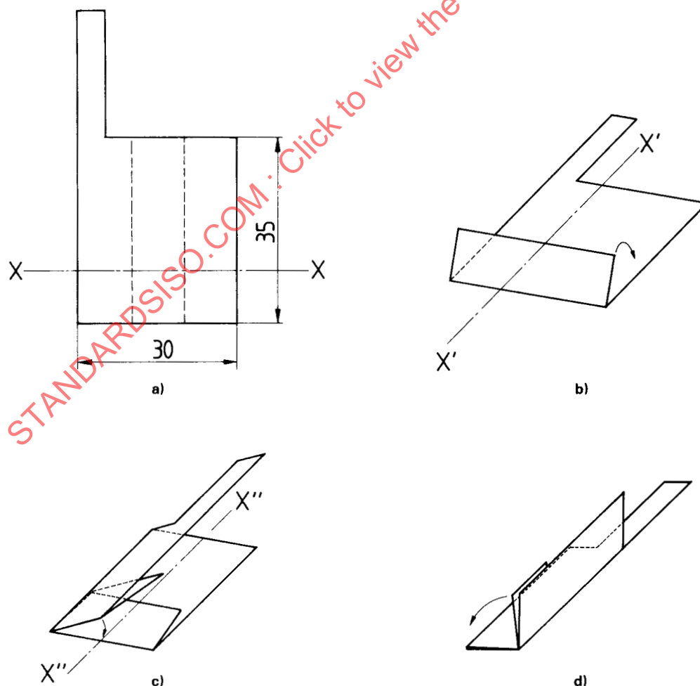
Figure 3 — Folding of filter paper containing test portion
