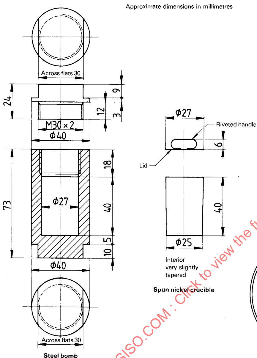
Figure 1 — Combustion bomb, gas-fired type (for method A)
