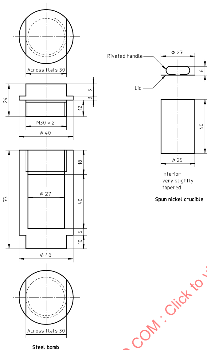
Figure 1 — Example of a combustion bomb, gas-fired type (for method A)
