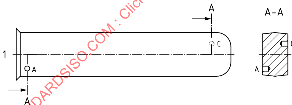
Figure A.5 — Sampling scheme for homogeneous vertical cast ingots or rectangular rods
