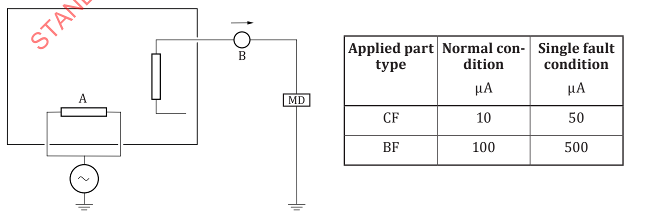
Figure 6 — Measuring circuit for patient leakage current from the patient connection to earth (Type Y)
