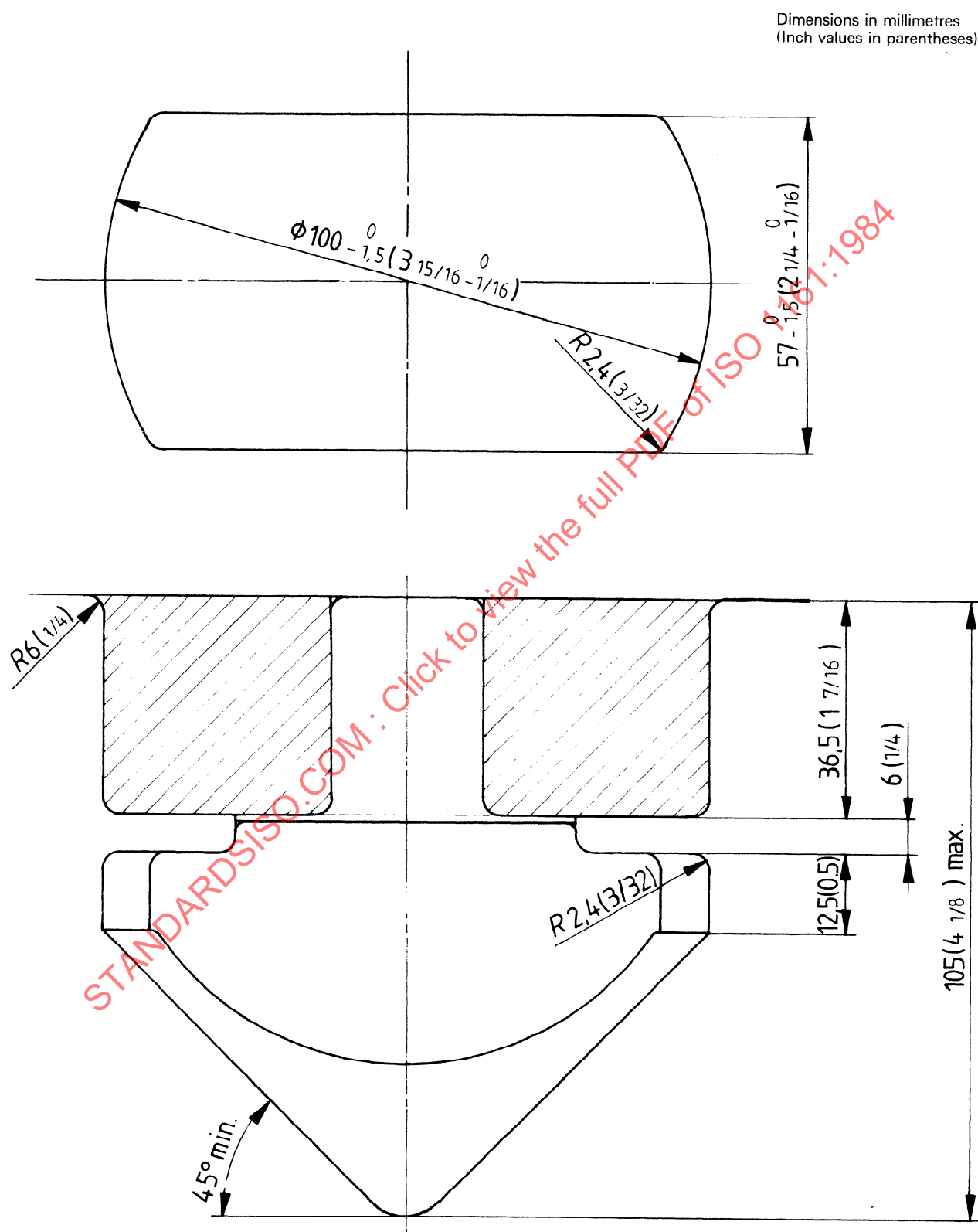
Figure 8 — Example of parallel-sided twistlock
