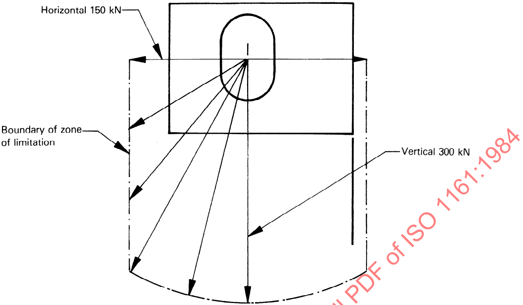
Figure 5 — Limits of loads due to lashing and securing
