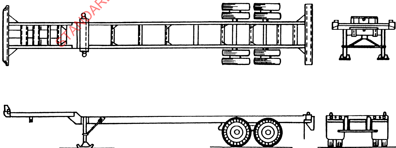
Figure 10 — Typical gooseneck container chassis
