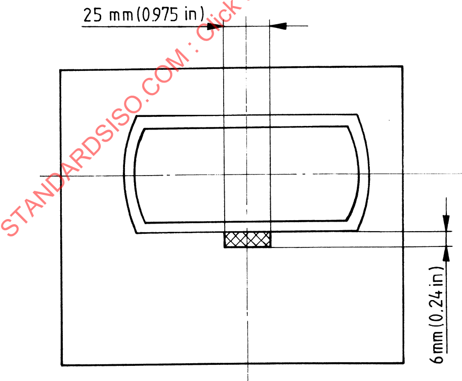
Figure 6 — Bottom view of bottom corner fitting showing contact area (shaded) for misgather (push-up) load
