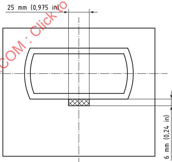
Figure 6 — Bottom view of bottom corner fitting showing contact area (shaded) for misgather (push-up) load
