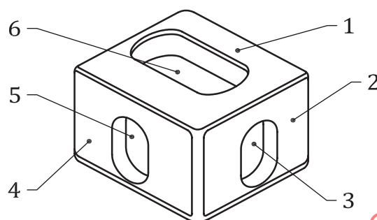
a) Upper corner fitting
