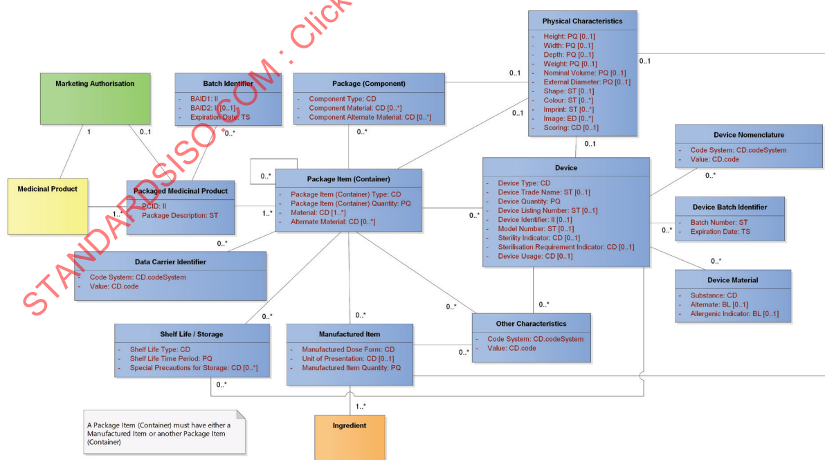
Figure 11 — Packaged Medicinal Product section detailed description diagram
