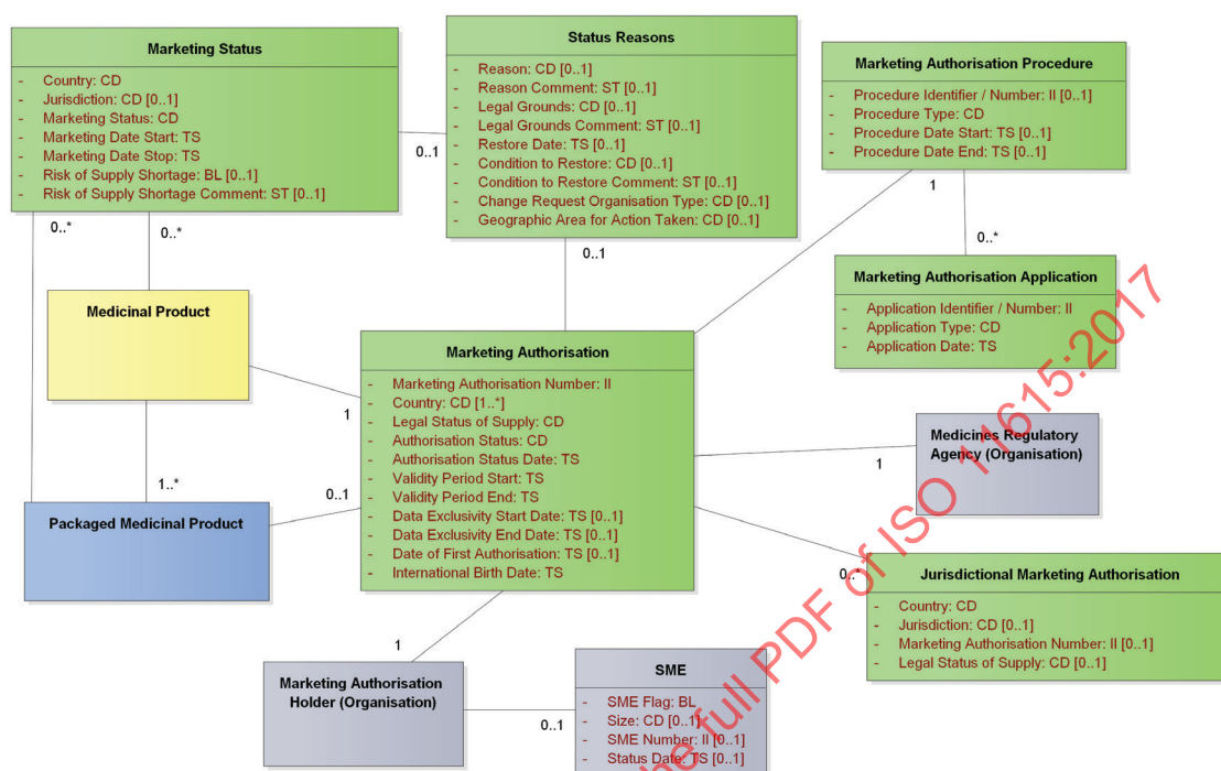
Figure 7 — Marketing authorisation section detailed description diagram
