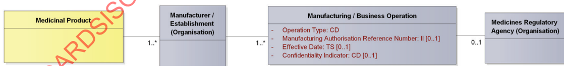
Figure 10 — Manufacturer/establishment section detailed description diagram
