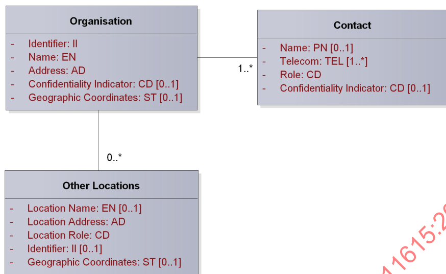
Figure 8 — Organisation detailed description diagram
