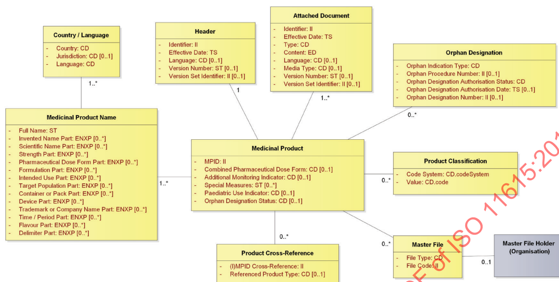
Figure 6 — Medicinal Product section detailed description diagram
