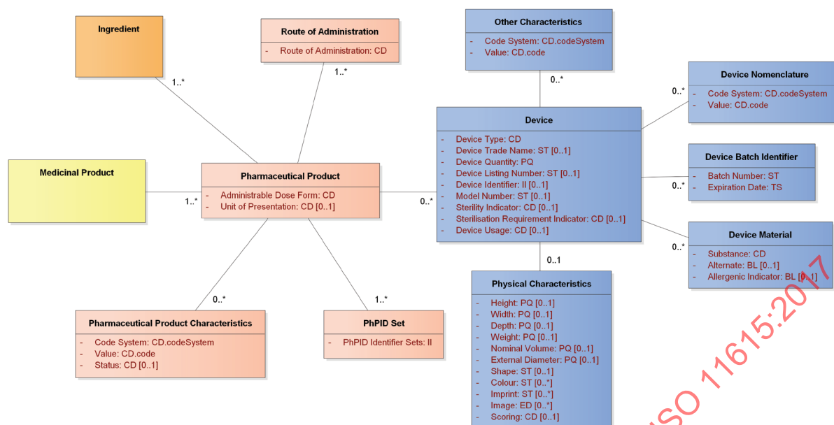
Figure 13 — Pharmaceutical product and device section detailed description diagram
