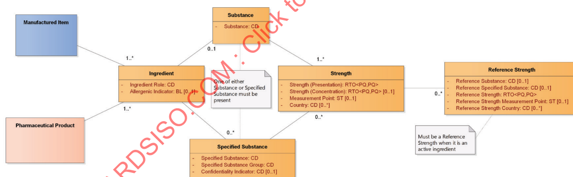
Figure 12 — Ingredients, substance and strength section detailed description diagram
