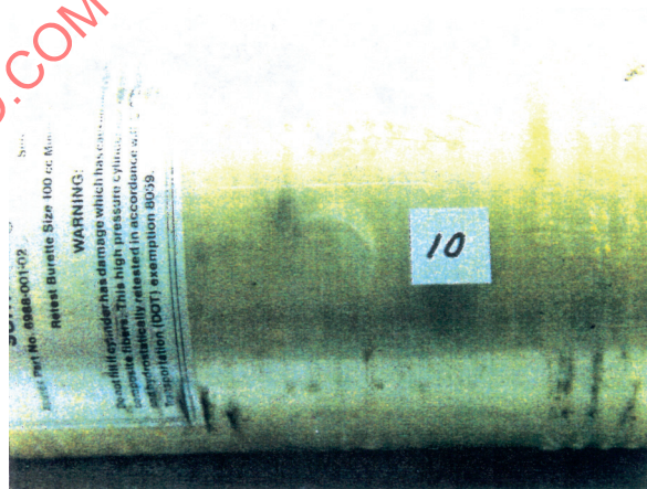
a) Level 1 impact damage — Superficial impact damage
