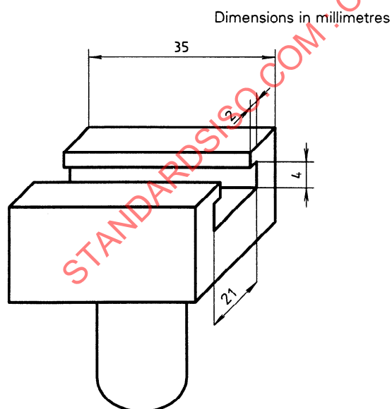
Figure 1 — Adherend-plate holder
