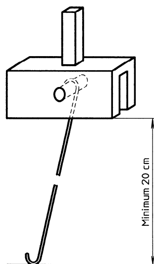
Figure 2 — Hook link
