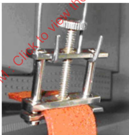
Figure 3 — Flat-jawed clamp
