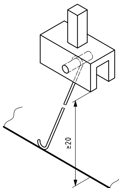
Figure 2 — Hook link
