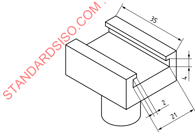
Figure 1 — Adherent plate holder ( \pm 2 mm for 35 mm, otherwise \pm 1 mm)
