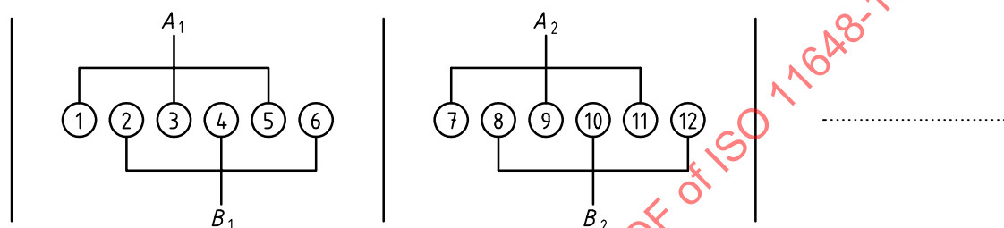
Figure 3 — Interpenetrating sampling
