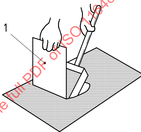
d) Outline of taking an increment by using a bump plate shown in c).
