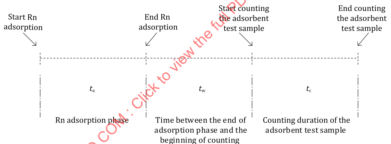
Figure 4 — Successive different steps of measuring process with their respective duration symbols
