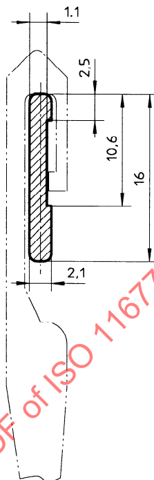
Figure 2 — Cross-section of heald-carrying rod for flat steel healds with J-shaped end loops
