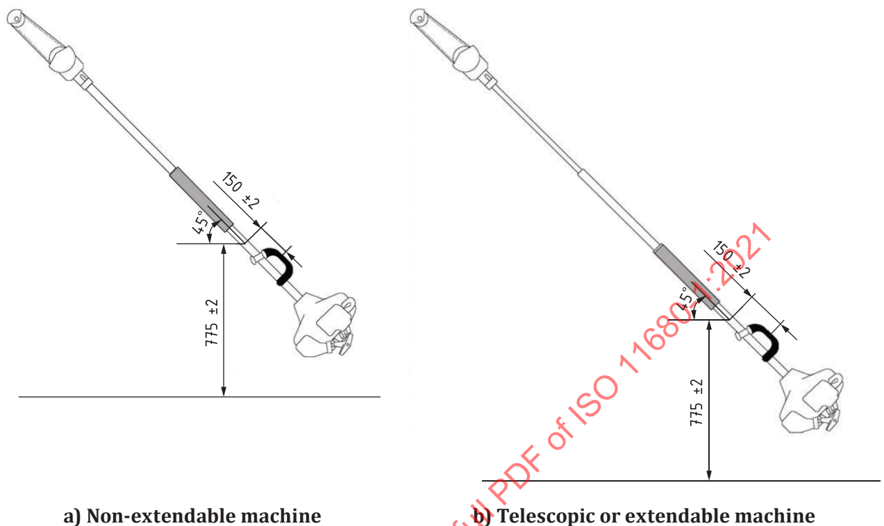
Figure 3 — Test set-up cutting attachment strength
