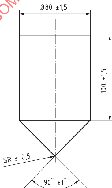
Figure 6 — Test cone
