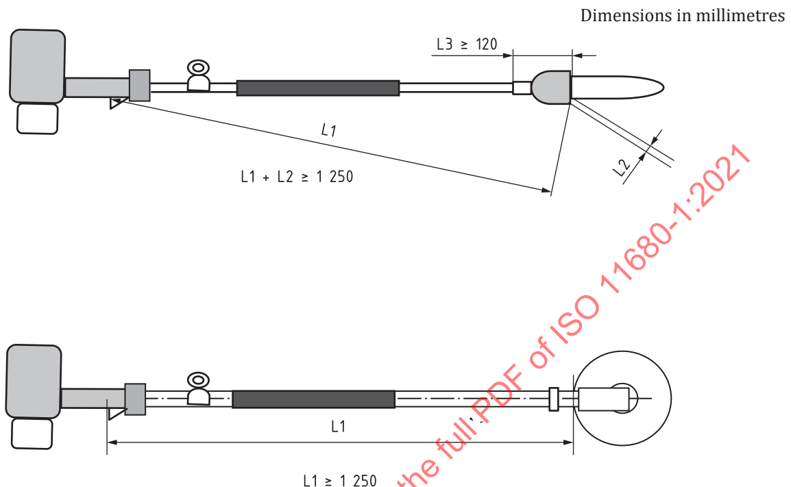
Figure 4 — Distance to the cutting attachment
